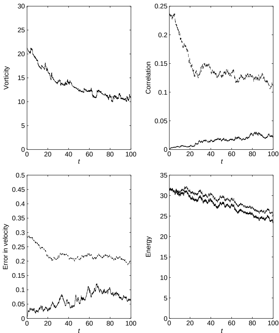
Figure 12.21 Comparison with crude closure dynamics during bombardment with localized vortices of alternating sign and amplitude equal to 5% of initial maximal vorticity |\omega|_{\max} \simeq 21.1 , with Newtonian dissipation \nu = 0.001 . Top left: maximal vorticity |\omega|_{\max} ; top right: correlation deficit \text{Corr-d}(\omega, \sinh(b\psi)) (plain) and \text{Corr-d}(\omega, \psi) (dashed, upper curve); bottom left: error in velocity \text{Err}(\vec{v}, v^*) using the point-vortex (plain) or the energy–enstrophy theory (dashed, upper curve); bottom right: energy E (plain) and approximate energy \bar{E} predicted by the energy–enstrophy theory (dashed, upper curve).
