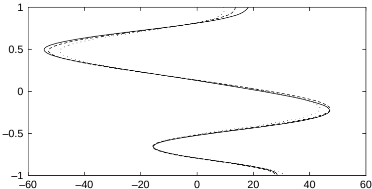
Figure 13.5 The Limage profile (solid) in the southern hemisphere band, and the zonally averaged velocity profiles for the equilibrium states with \varepsilon = -0.02 (dashed) and \varepsilon = -0.035 (dotted).
