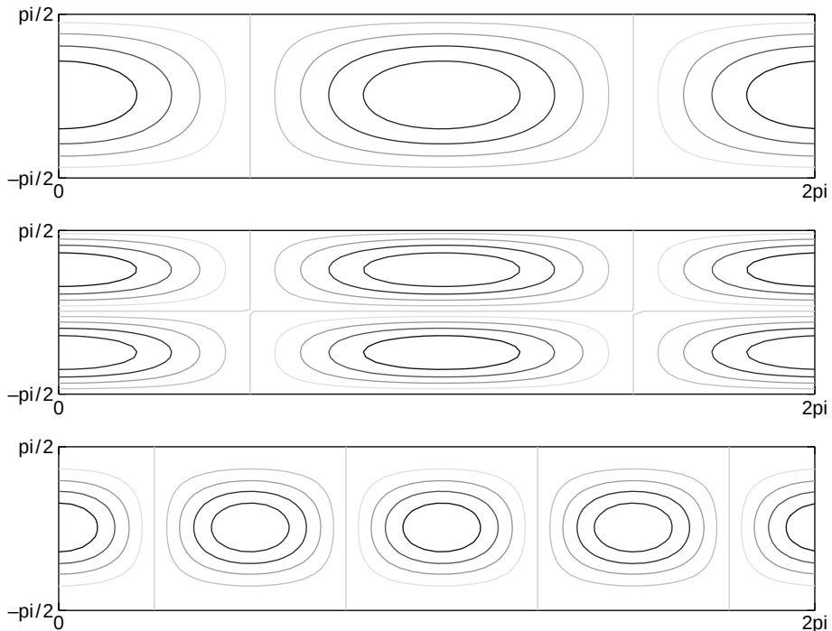
Figure 16.2 Surface spherical harmonics corresponding to spherical Rossby waves in moving frames. Top: \cos \theta \cos \phi , n = m = 1 ; middle: \cos \theta \sin \theta \cos \phi , n = 2 , m = 1 ; bottom: \cos^2 \theta \cos(2\phi) , n = m = 2 .
