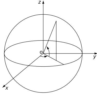
Figure 16.1 Spherical coordinates.
